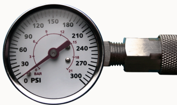
Pressure Gauges
